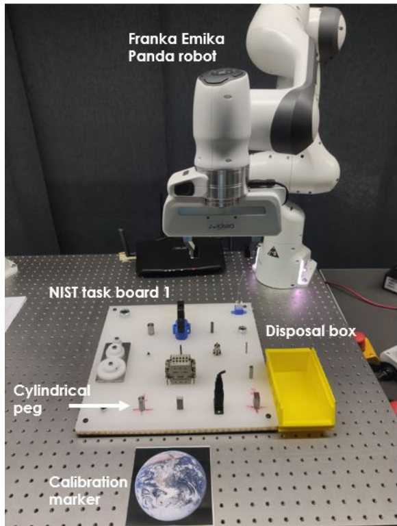
Fig. 7: Experimental setup with Franka Emika robot, NIST board, calibration marker and disposal box.
